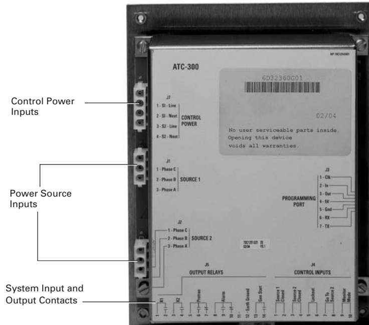
Rear View of ATC-300 Automatic Transfer Switch Controller
